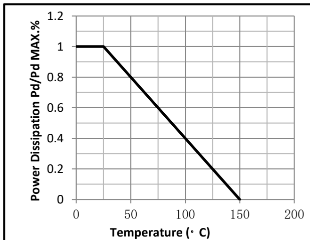
Fig.3 Power Dissipation
