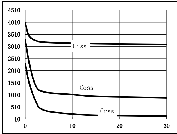
Fig.2 Capacitance Characteristics
